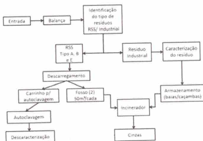
Figura 2 – Fluxograma PGRSS
